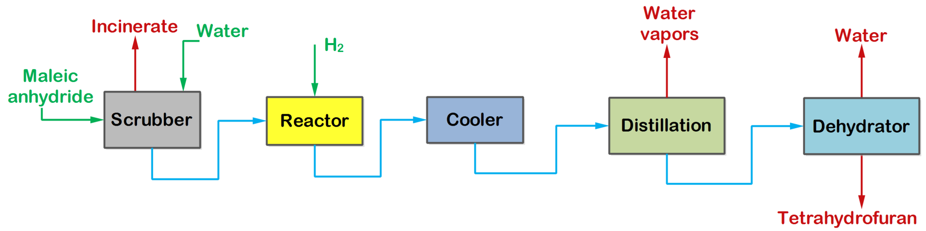
Figure: Manufacture of tetrahydrofuran by maleic anhydride hydrogenation
